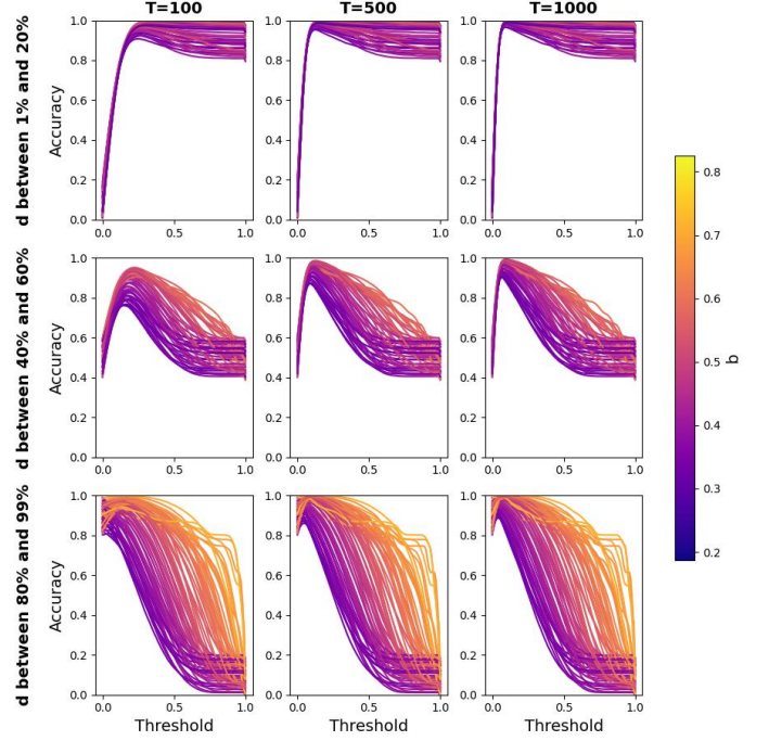
Fig. 3. Accuracy obtained when applying different thresholds on an empirical correlation matrix, depending on the graph density d , the number of observations T , and the mean value of the non-zeros coefficients b .
