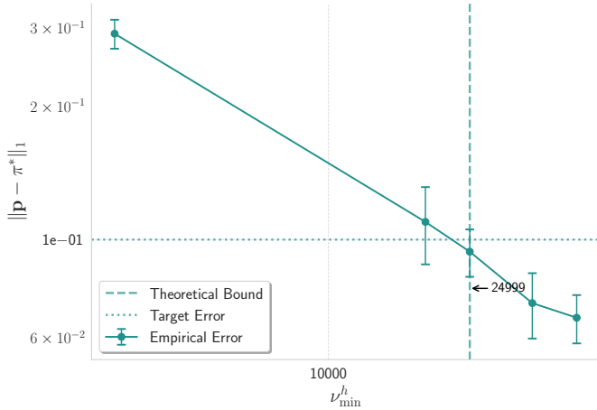
Fig. 3. Sample complexity analysis for \epsilon = 0.1 , showing increased sample requirements for lower error tolerance.
