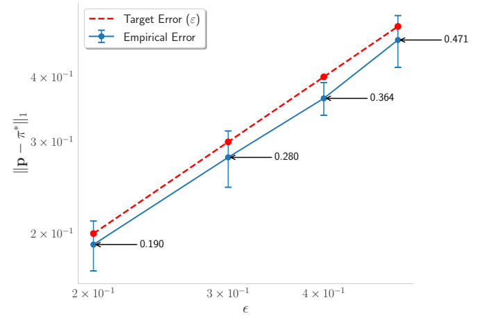
Fig. 1. Empirical approximation error versus theoretical thresholds for varying \epsilon values. Error bars represent standard deviation across 10 random seeds.
