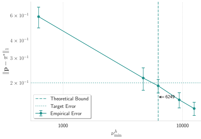
Fig. 2. Approximation error as a function of high-return samples for \epsilon = 0.2 . Vertical line indicates theoretical minimum sample size.
