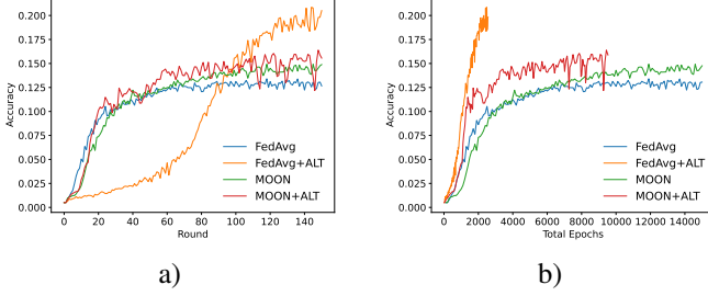
Fig. 4. Accuracy curve on Tiny-ImageNet: a) per round; b) per total number of training epochs.
