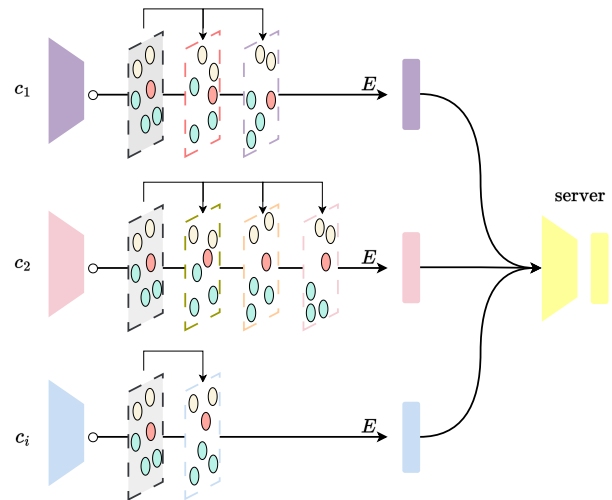
Fig. 1. Overview of the proposed federated learning strategy with dynamically changing local training epochs. At each communication round, clients perform a variable number of local epochs, different between each others, depending on their feature representation. As an example, in the figure the second client performs more local epochs than the other clients.
