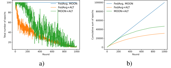
Fig. 3. Training length on the CIFAR-10 dataset: a) Total number of epochs performed at each round; b) cumulative sum of the performed epochs during training
