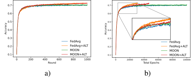
Fig. 2. Accuracy curve on the CIFAR-10 dataset: a) per round; b) per total number of training epochs.
