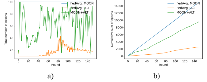
Fig. 5. Training length on the Tiny-ImageNet dataset: a) Total number of epochs performed at each round; b) cumulative sum of the performed epochs during training.
