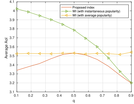
Fig. 3. Average AoI vs q for two other popularity modes.
