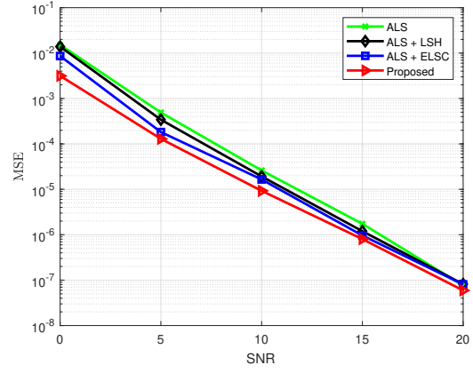
Fig. 1. Channel estimation MSE versus SNR comparison.
